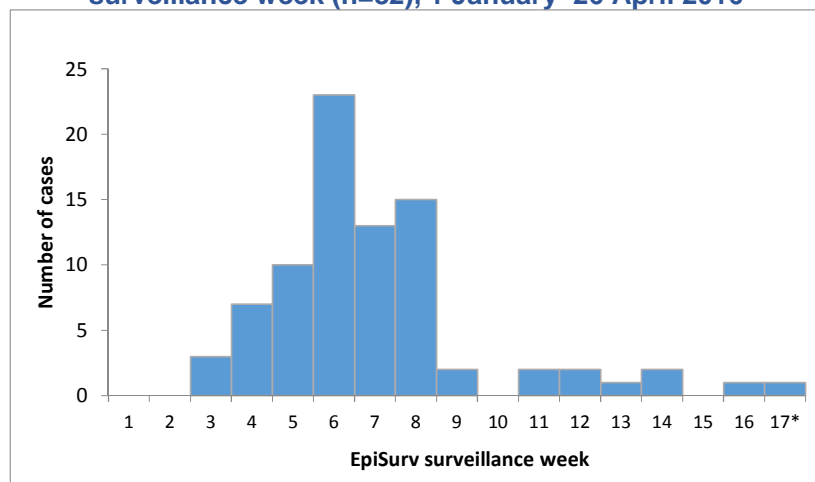
Figure 1. Zika virus infection (confirmed) cases notified in New Zealand by EpiSurv surveillance week (n=82), 1 January–26 April 2016
